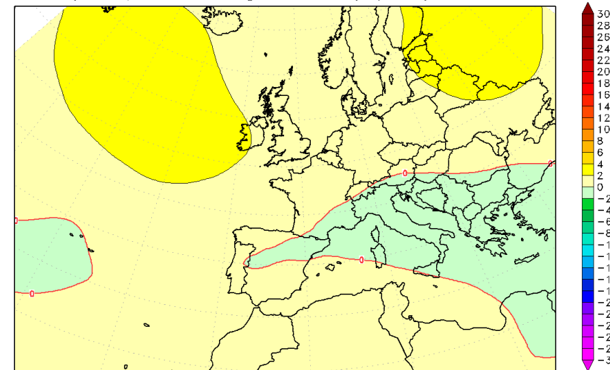
ECMWF weekly forecast A_0400 Mon 11JUL2022 00UTC 25dy FC AN: 2022061600
